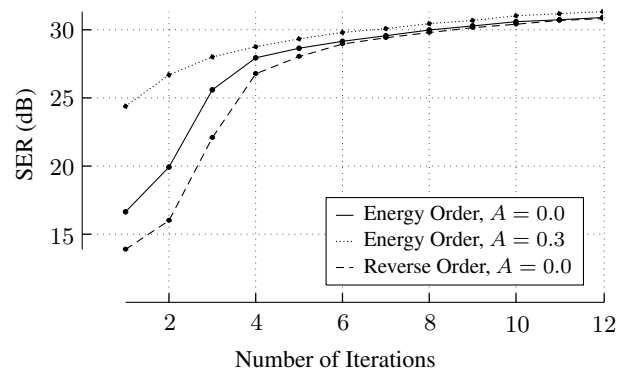
Figure 8: SER values vs the number of iterations. Single-resolution RTISI, block size 2048 samples.
