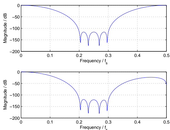
Figure 5: Frequency responses of the input filters of the two hyper-meshes used in the room impulse response simulation: above for the mid frequencies and below for the highest frequencies.
