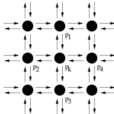
Figure 1: A two-dimensional rectilinear DWG mesh structure. p_k is the junction currently calculated and p_l , where l = 1, 2, 3 , or 4 , are its axial neighbors as in (8).
