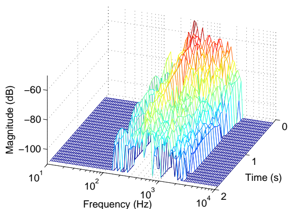
Figure 11: Combined response of the two hypermeshes used in the simulation of the clavichord soundbox impulse response. The low-frequency modes implemented with separate resonators are not included.
