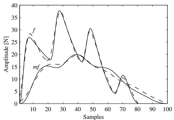
Figure 2: Hammer filter design: the target response F(n) (solid line) and the impulse response of the hammer filter H_h(z) (dashed line) for playing forte and mezzoforte (the latter is multiplied by a factor of 5 for picture clarity) on a C_4 string.
